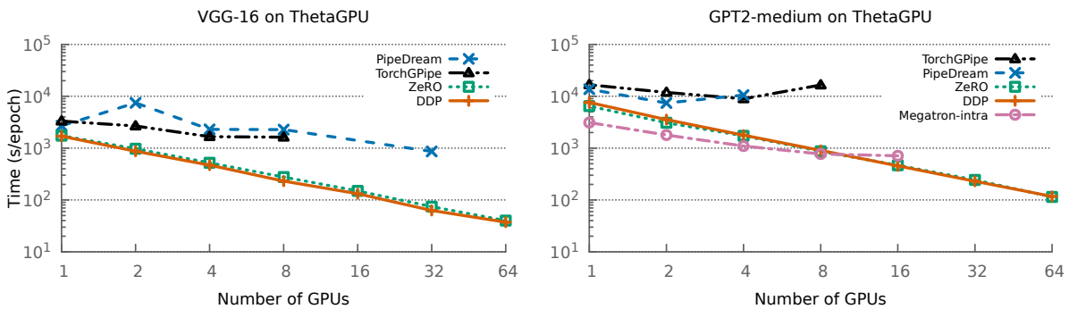
Figure 7: Performance results on ThetaGPU for VGG-16 and GPT2-medium.
