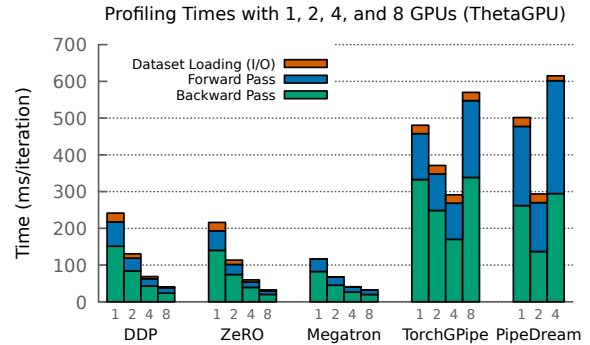
Figure 5: Breakdown of time spent in training on 1, 2, 4, and 8 GPUs of ThetaGPU for GPT2-medium. We use NVIDIA’s NVTX SDK for annotating events and Nsight Systems for instrumentation. Megatron refers to Megatron-intra.
