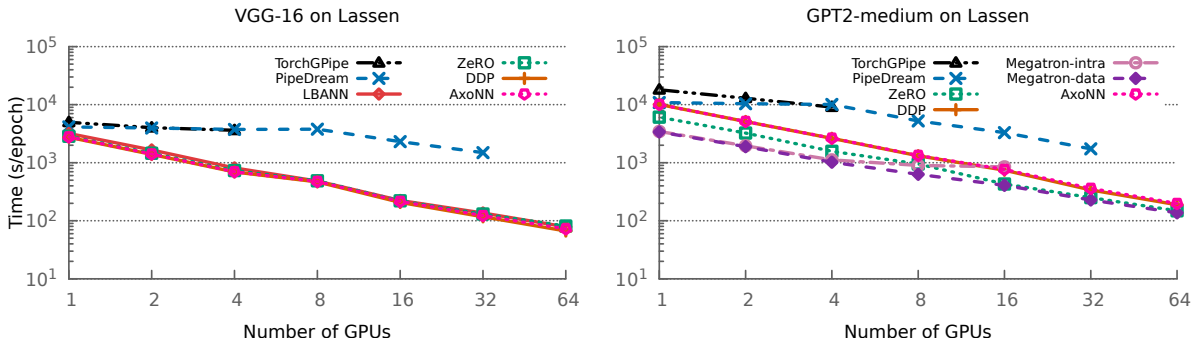
Figure 6: Performance results on Lassen for VGG-16 and GPT2-medium.
