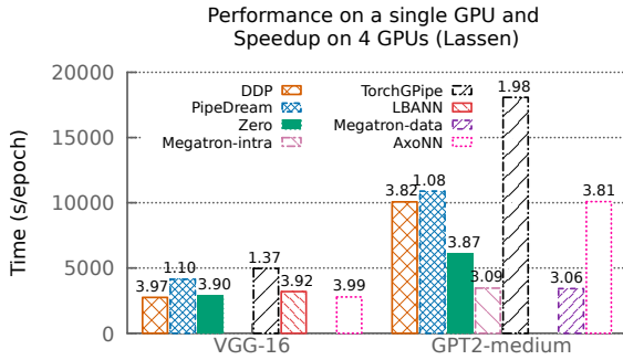
Figure 4: Comparison of single GPU performance and 4 GPU speedup on Lassen for VGG-16 and GPT2-medium. The labels list the speedup of each framework relative to their own 1 GPU performance.
