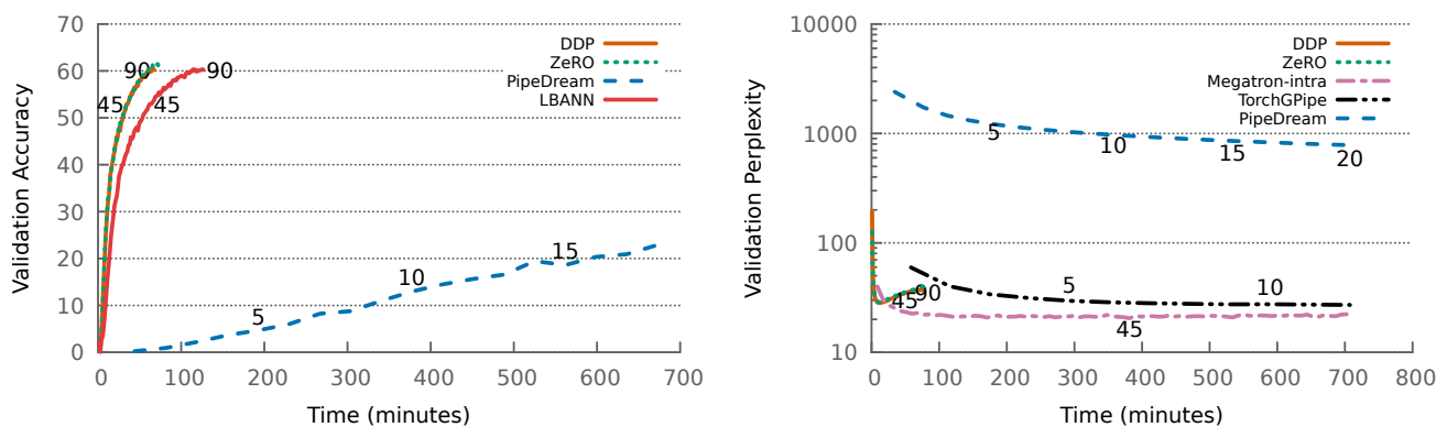
Figure 8: Validation performance by time for training VGG-16 and GPT2-medium on ThetaGPU. Epoch numbers are shown in labels.
