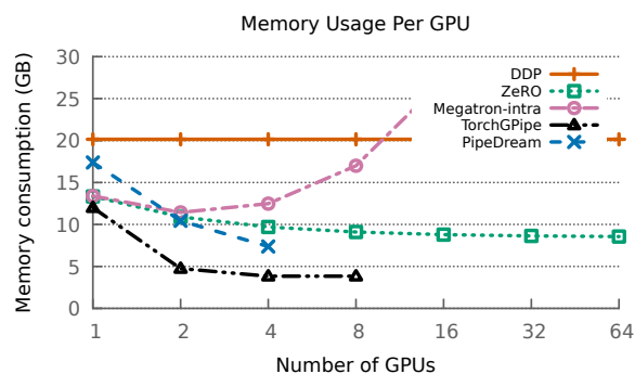
Figure 9: Memory consumption by different frameworks on ThetaGPU for GPT2-medium.
