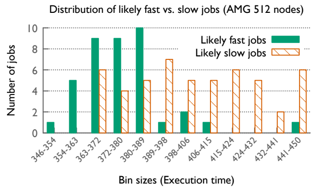
Fig. 11. Distribution of actual runtimes of likely fast versus slow jobs of AMG when considering above median values of three features: RT_STL_COL, RT_STL_GBL, and NUM_GROUPS
