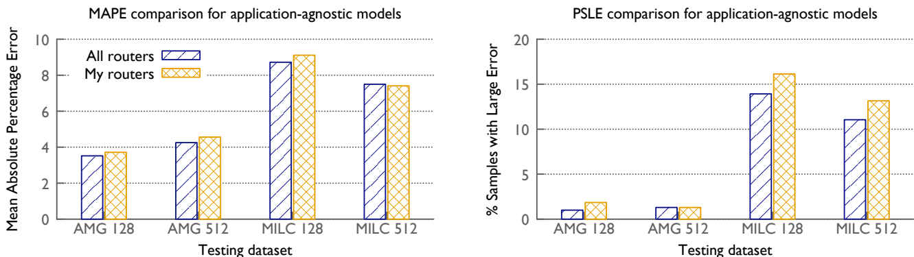
Fig. 8. MAPE and PSLE scores for the NN model when using three datasets for training and a fourth disjoint dataset for testing (x-axis label.) The training dataset for each cluster is the combination of AMG 128, AMG 512, MILC 128, MILC 512 minus the dataset in the x-axis label.
