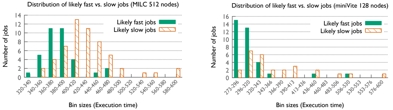
Fig. 12. Distribution of actual runtimes of likely fast versus slow jobs of MILC and miniVite when considering above median values of three features: RT_STL_COL, RT_STL_GBL, and NUM_GROUPS
